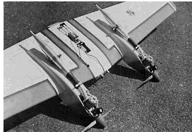
It's really a simple design, yet exotic in line and color. Nacelles build up quickly, soak up the vibration and stress. It's performance is astonishing. At top: Pushrods to the rudder and elevator exit neatly, transmit the motion without snaking around and losing servo power. Note ample tail area.
