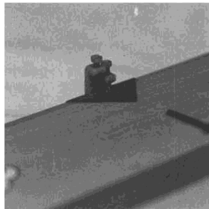
Stab in place, with V.I.T. arms in locked position. Screws hit plywood seat.
