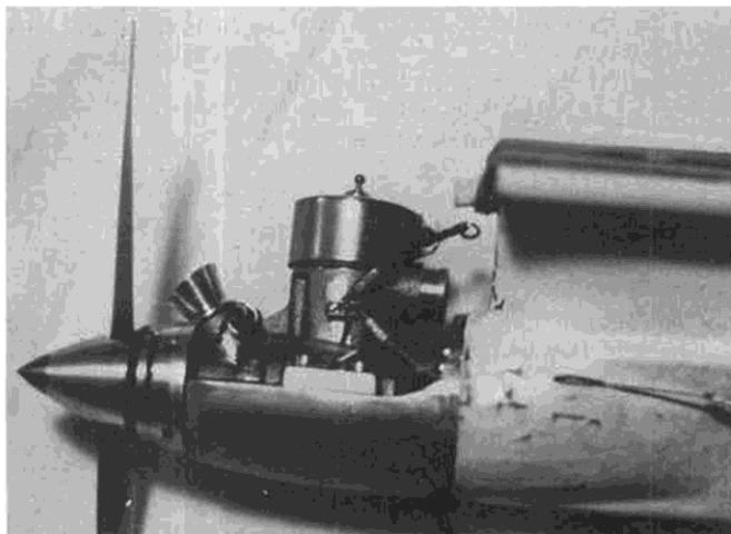
Left side view showing cylinder muff, flood-off switch, and engine brake installation. Monks timer.
