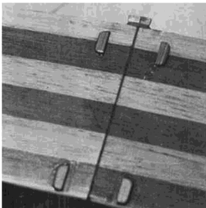
Wing keying blocks and plywood rubber band connector that keeps panels together.
