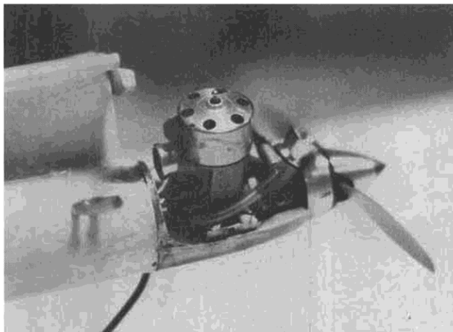
Rear side view of engine compartment and tank filler tubes. Metal "muff" speeds heat-up of engine after starting, for quicker launches.
