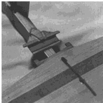
Stab mounting system. Accurate indexing system provides consistent alignment.
