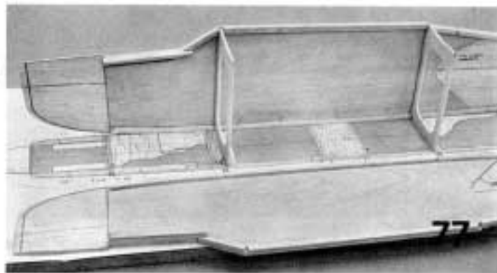
77. Pin the fuselage side to the top view plan along the flat part between F-2 and the back of the landing gear plate.
