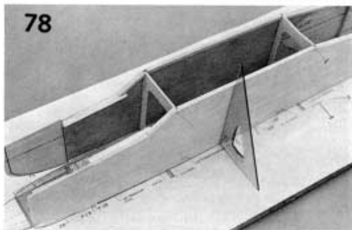
78. Epoxy glue the remaining side to F-2 and F-3. Pin in place and check for square with a triangle.
