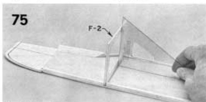
75. Put 5 minute epoxy on F-2 and glue in place. As the glue sets up, use a triangle to get F-2 exactly perpendicular. Other glue can be used if you secure the former in place while it is drying.
