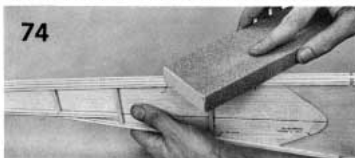
74. Finish the side to exact contour by use of the sanding block. Place the two sides together and match them by sanding as required to make them duplicates.
