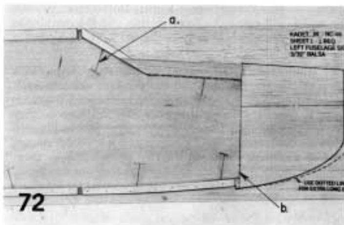
72. a. Pins around the edges can help hold down the doubler during the set up or drying process.
