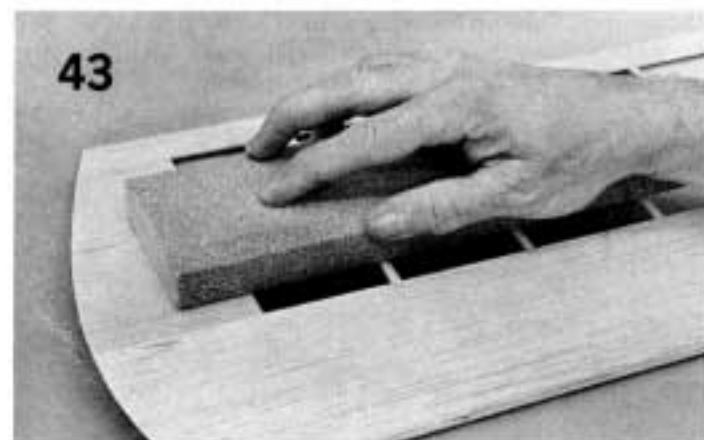
43. Sand the top of the cap strips and tip planking even.
