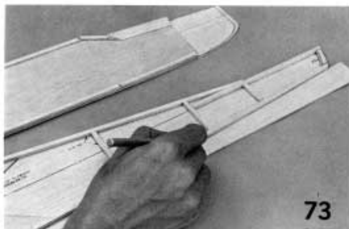
73. Cut the fuselage sides from the sheet with a modeling knife. Don't cut too close, leave a bit for sanding, cutting too close can result in too deep a cut that is harder to fix than taking down the side a little with the sanding block.
