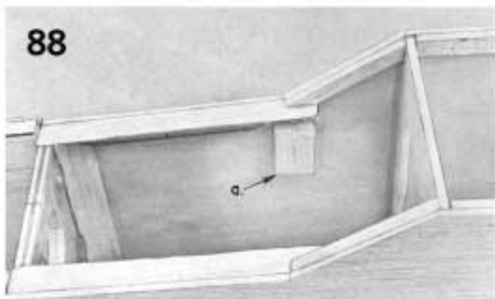
88. a. Place small blocks on each side of the fuselage to hold the tank centered. Don't get the blocks too tight, just enough to keep the tank from rattling around and yet release the tank easily for removal when needed.
