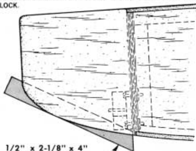
129. Fit the \frac{1}{2} " x 2\frac{1}{8} " x 4" bottom nose block into place. OIL-PROOF THE FIREWALL FACE AND INSTALL NOSE GEAR BEARING SEMI-PERMANENTLY BEFORE GLUING ON BOTTOM NOSE BLOCK.
