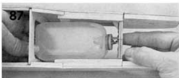
87. Practice passing the assembled tank through F-2 and make sure that it can be passed in and out of the fuselage nose after the fuselage is closed up. If there is any problem that hinders easy insertion and removal of the tank, fix it now while access to the nose is easy.
