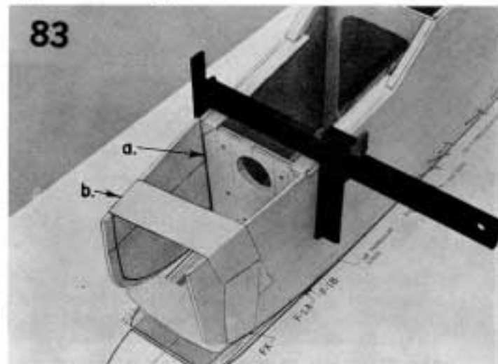
83. a. Put epoxy glue on both sides of the firewall F-1.
