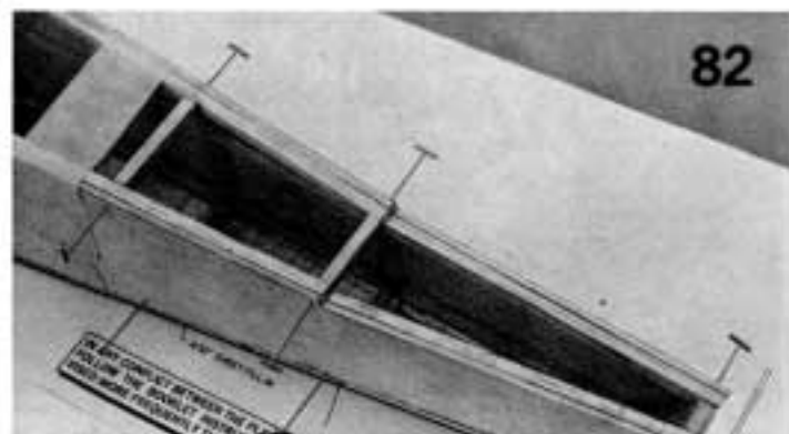
82. Use pins and masking tape to hold the fuselage together until the glue dries.
