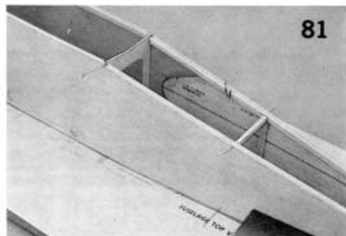
81. Pin and glue the remaining rear fuselage cross pieces in place.
