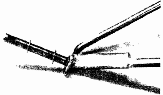
Brass tube is used for the solder joint instead of soft wire. Very strong. Note flat ground for wheel collar retaining screw.
