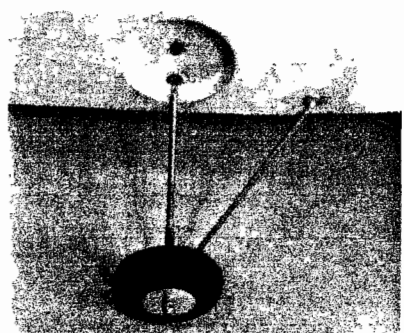
The finished assembly installed on the fuselage.
