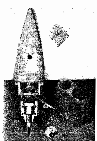
Hatch in nacelle allows easy access to throttle servo. Note hole for servo cable. Four screws retain the engine cowling.
