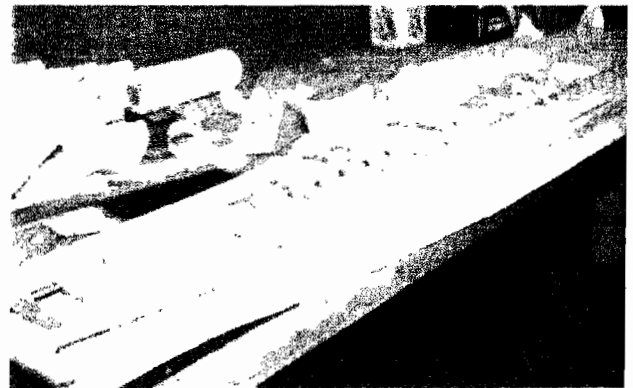
A paper tube will be inserted into holes in ribs to allow easy installation of servo cables. Shear webs run full span on both the front and rear spars. The engine mounts are tied into the main structure.
