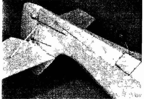
Steerable tailwheel is easily removed and replaced with a water rudder. Note the diagonal braces to the horizontal stabilizer.
