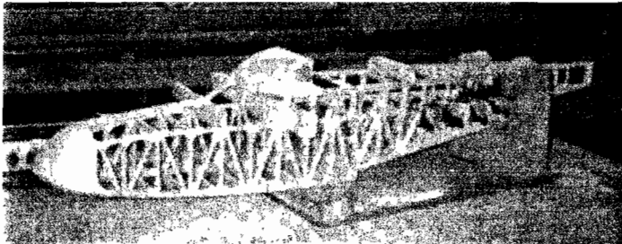
The top cabin block must be supported in position while the cement cures. Then, add the balsa nose block and rear fuselage (turtledeck) formers.
