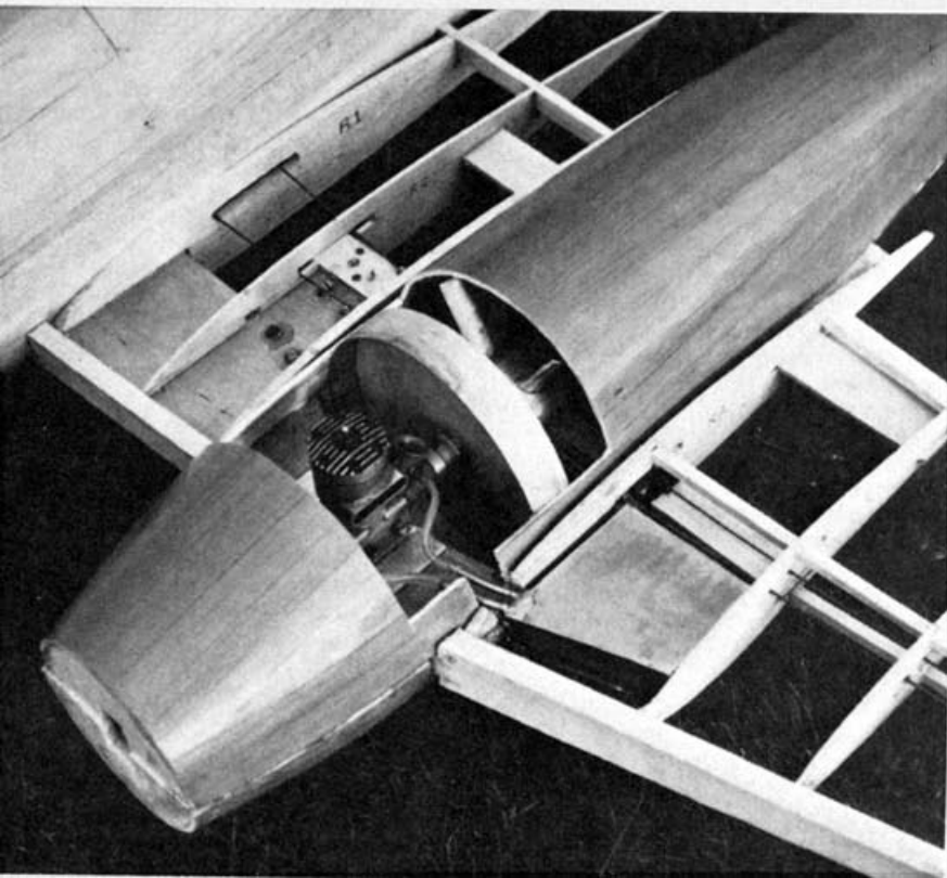
ABOVE: The rather big wheels on the model are actually scale. Obviously, they produce gobs of drag. Retracts would help performance as well as the jet impression. LEFT: Engine sits on an aluminum plate sandwiched in a plywood mount. This must be exceptionally rigid. Any vibrations could cause the fan to hit its shroud with disastrous results. Note fuel tank location in the wing.
