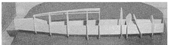
Basic fuselage structure.
