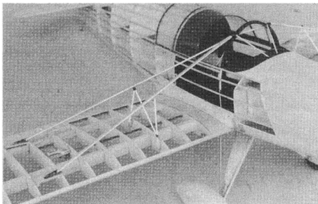
Strut details. Note fillet construction.
