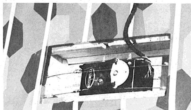
View of aileron servo linkage.
