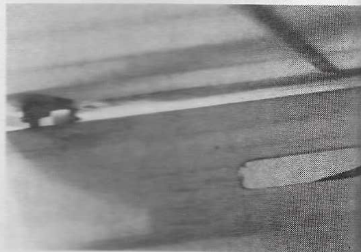
Stabilizer is adjustable near its leading edge. Could be controlled by another servo if you wish to go first class. Elevator pushrod, right.
