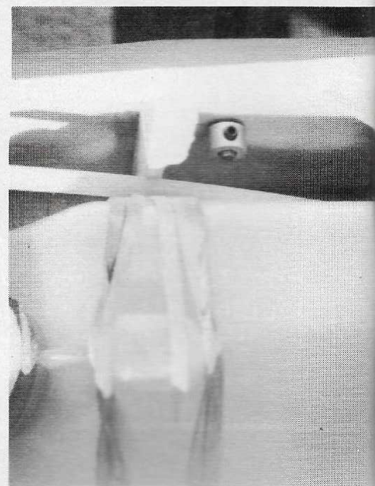
The 8 oz. slant tank gives plenty of capacity for long flights. Here, rubberband hold-downs pass in front and in back of bubble on top.
