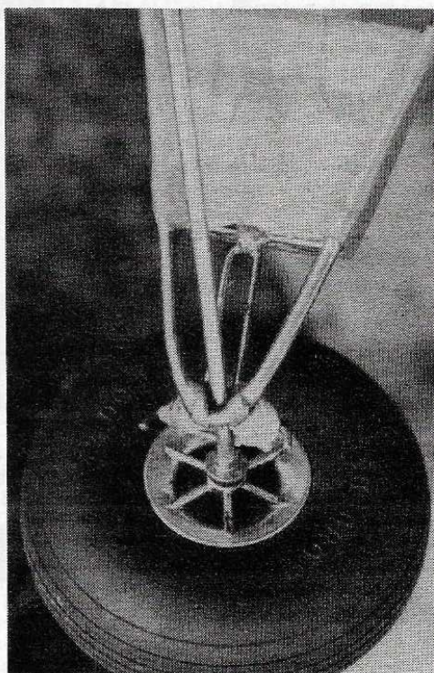
Practical shock absorbing uses rubber as bungee cords. Landings consequently are quite soft.
