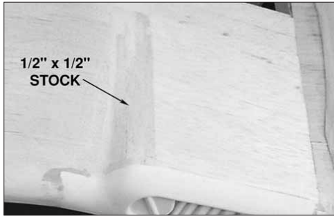
□ 4. Use leftover 1/2" x 1/2" balsa hinge block material to fair in the outboard ends of the oil coolers.
