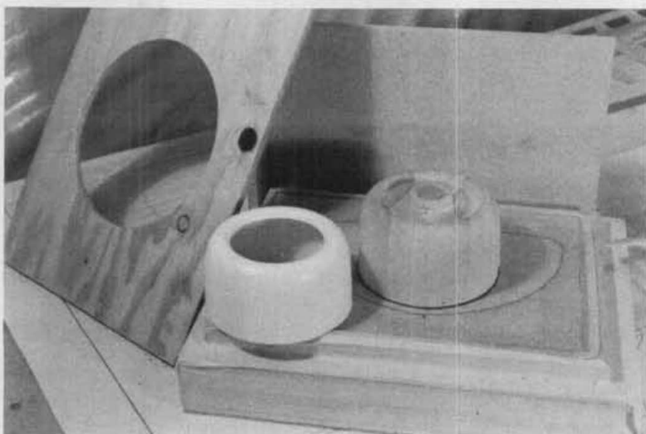
Vacuum former, plug, and finished cowl. Cowl can also be made from fiberglass, or built up in the usual way from balsa wood.
