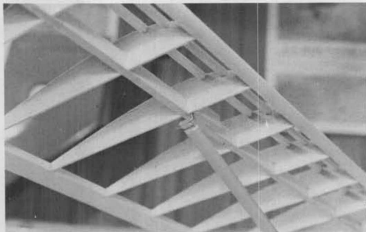
Wing strut mount is simple and clean. Struts are 1/4x1/2 spruce.
