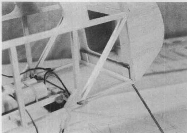
Close-up shows the strut attachment and landing gear installation.
