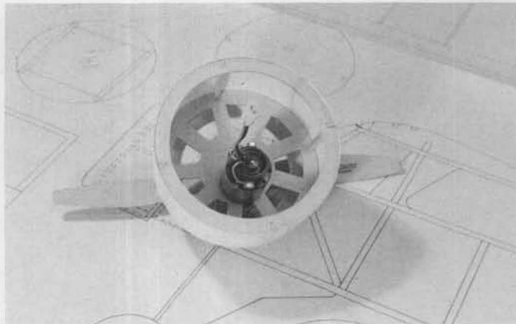
Back view of cowl shows Leisure geared motor installation.
