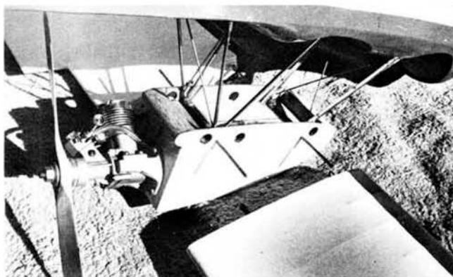
View of underside of center section, with wing panels ready for hook-up. Note left hand prop which was hand carved. Not really difficult.
