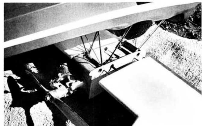
Right wing is now attached, aileron clevis hooked to crank. Wing held on by rubber bands to cup hooks. Power is Enya .35.
