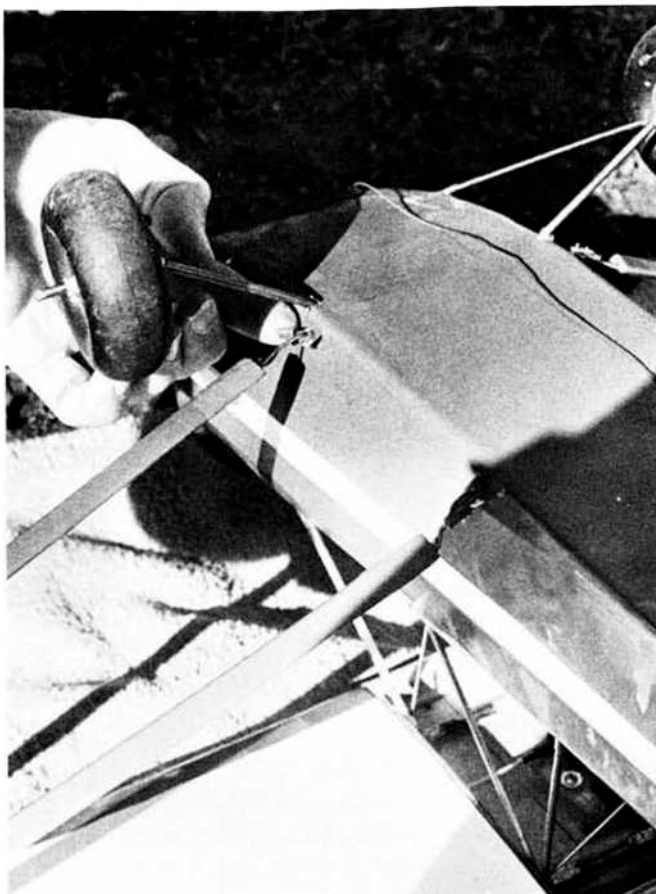
Functional wing struts are hooked on using Rand keepers. "Z" bend in 1/16 inch wire provides adjustment for length. Note receiver antenna.
