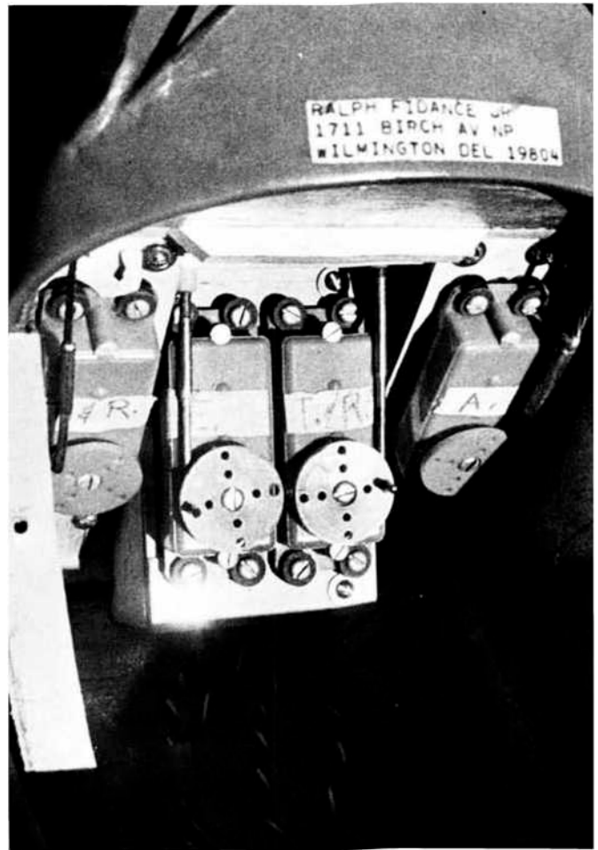
The "office" with Micro-Avionics servos. Outboard servos move cables leading to throttle and aileron controls in engine nacelle. Simple rig.
