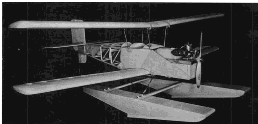
The uncovered airframe (and water frame?) of the PT-1 reveals the wide wing spacing and the uncowed motor . . . like the full-size version. Foam wings could also be used.
