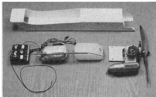
Bare fuselage is shown with O.S. .32 engine, engine mount plate, 4 oz. slant tank, receiver/battery switch assembly, and servo assembly for radios, with elevon mixing capabilities.
