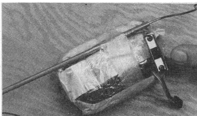
Receiver-Battery switch assembly is wrapped in foam, covered with plastic wrap (to protect against oil and fuel), and taped up. Outer NyRod extends past fuel tank to engine, allowing a free passage for the throttle pushrod.
