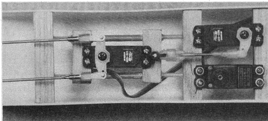
A simple sliding tray may be built from NyRod scraps and plywood. Inner NyRod is also supported with 1/16" music wire inside. Servo rails are screwed in from outside of fuselage.
