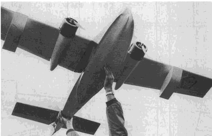
Underside shot discloses the wide hull and spray rails which help prevent water spray from hitting the propellers during takeoff runs. Wide tip floats not as pretty, but very functional.
