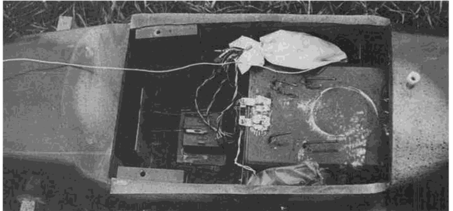
Endurance anyone? Though it will hold a gallon tank, this one is a mere 5 pint fuel cell, which supplies the individual 9 ounce nacelle tanks through engine pressure. Lots of radio room.
