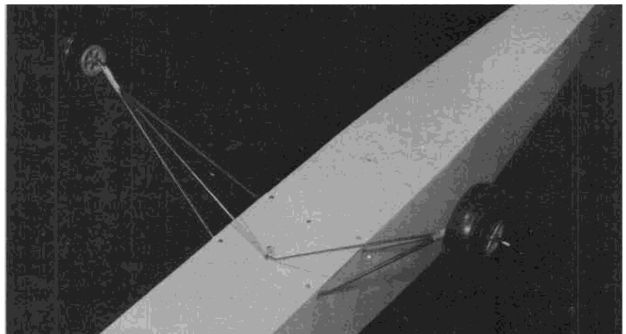
Main gear installation. Struts fit into grooves in hardwood blocks in fuselage, are held captive by a removable plywood plate.
