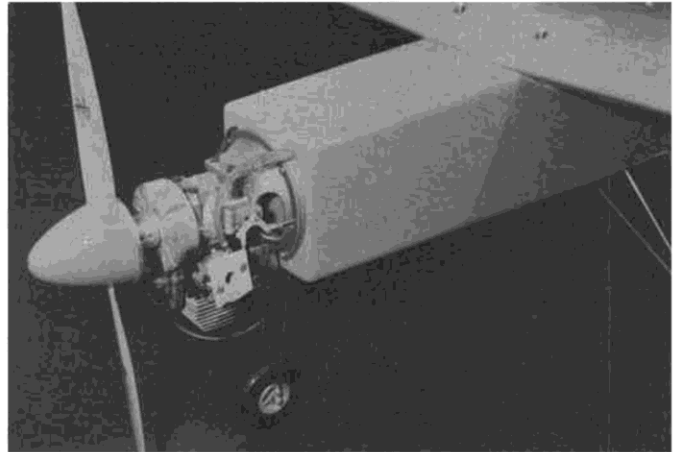
Plywood hatch allows easy access to tank. A cowl would be nice, but wouldn't be in keeping with the Ugly Stik tradition.
