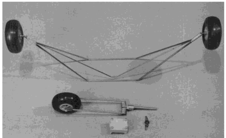
Main and nose gear, bent and ready to install. Nose gear is a non-standard item, has to be custom made. A simple job for your club machinist.
