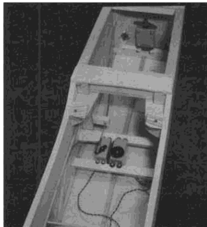
Throttle and nose gear servo installation. Plenty of room for a radio (and 3 or 4 more!).
