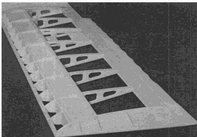
Ribs are 1/8 Lite-ply with balsa cap strips. Internal box spar, also 1/8 Lite-ply, preserves open-structure look.
