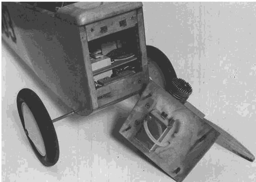
Super-sanitary tank and equipment installation. Note ballast servo-taped to mounting board. Externally operated switch in front. One ounce tank gives 6 minutes. No throttle used.
