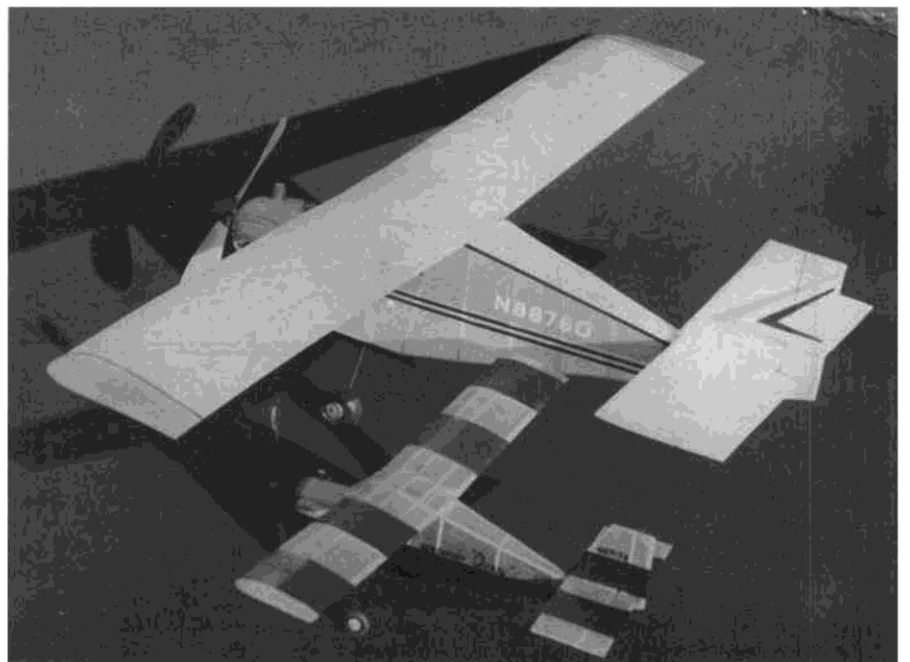
Father and son Quails. The large one is recommended for beginners because the larger wood sizes are easier to handle, and the large size also makes the big one easier to trim for flight.
