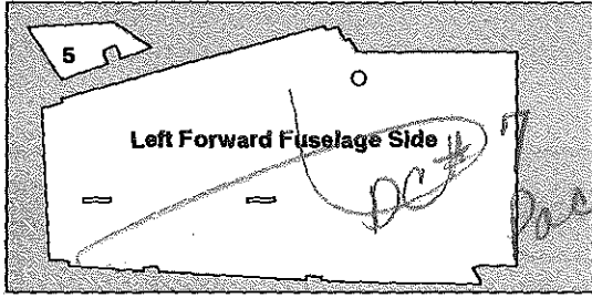
33320 - 1 REQUIRED - 3mm x 7-27/32" x 15-27/32" (3mm x 199mm x 402mm) - MICRO-LITE PLYWOOD
