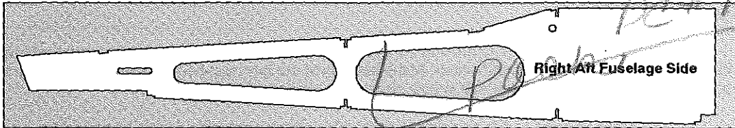
33321 - 1 REQUIRED - 3mm x 6-27/32" x 39-27/32" (3mm x 174mm x 1012mm) - MICRO-LITE PLYWOOD
