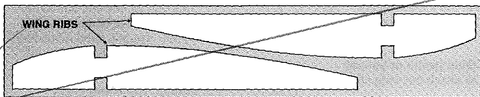
33343 - 13 REQUIRED - 3/32" x 2-7/8" x 14-7/8" (2.3mm x 73mm x 378mm) - Balsa
