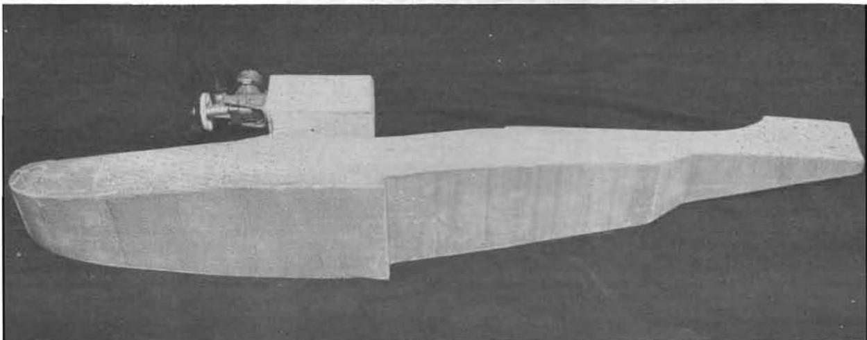
BELOW: Bottom and sides of hull have been glassed and resined.
