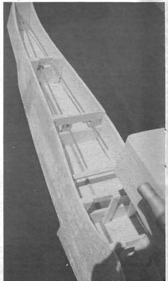
Hull is ready to close up the top. Plans show engine pod tapered at rear for improved looks.
