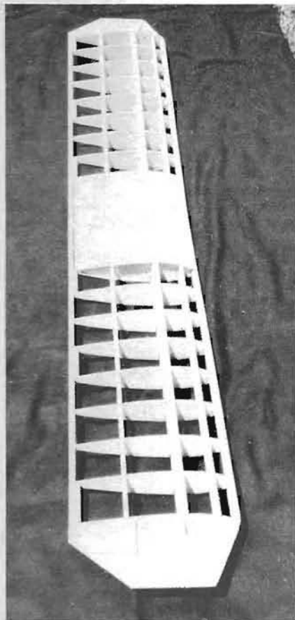
Basic wing all framed up.
