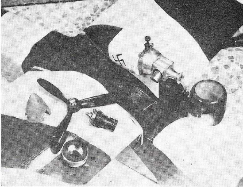
One-piece aluminium cowl on prototype necessitates removal of liner and muffler for fixing. Reinforced card could be used.
