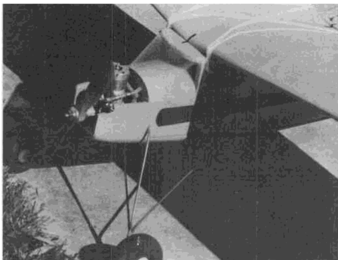
Power for Ron's "reduced" Dallaire is an Enya .29. SAM rules will allow up to a .35. No thrust offset.
