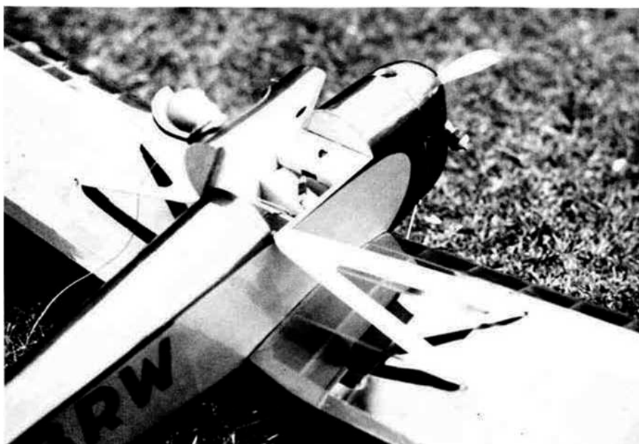
Access to the Stomper actuator. Commander receiver, and switch/battery pack comes with a flip of the hatch. Switch can be operated through the cockpit without disturbing the Roman pilot.
