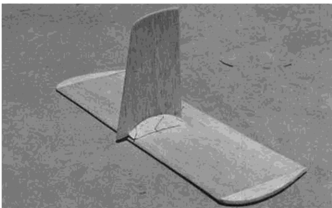
Stab assembly is a cinch. Triangular fin gusset is on left side only. Rudder is attached with figure-8 thread hinges.
